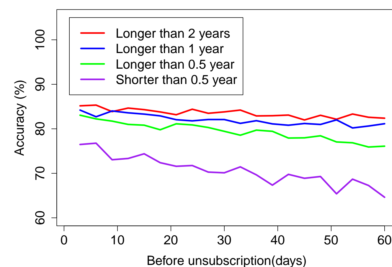
FIGURE 4: Predictivity of our classification method.
